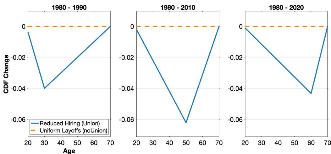
Figure 4: Change in CDF of age distributions relative to steady state in simulated thought experiment.
